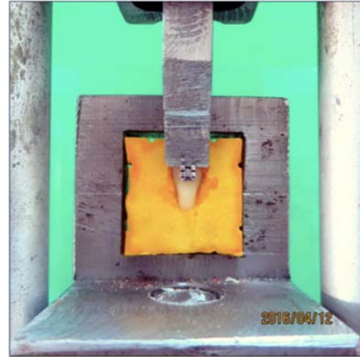
Figure 1: Specimen fixed inside holding apparatus, force at bracket-tooth interface until bracket detached. A computer, electronically connected to the testing machine, recorded the force to debond the bracket in Newton. The bond strength was calculated in Mega Pascal (MPa) by dividing the force (Newton) to the surface area of brackets in (mm 2 ), yielding the result at MPa.
